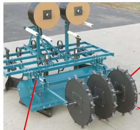
Hinge point allows frame to float
